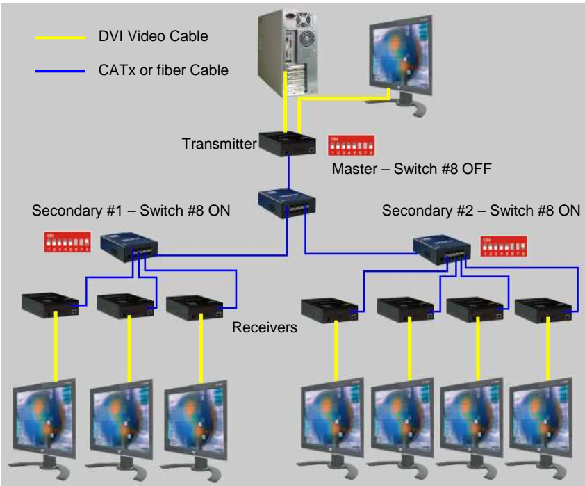
Figure 4. Multiplex Repeater (Cascaded configuration)
