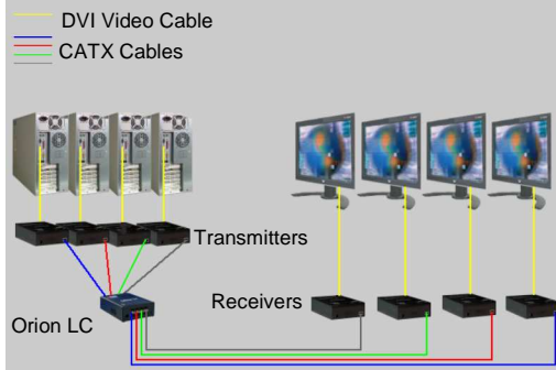
Figure 3. Multiplex Repeater 4x4
