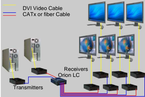
Figure 2. Multiplex Repeater 2x3
