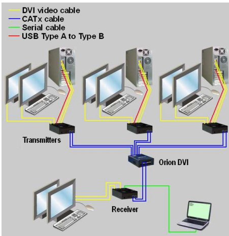
Figure 14. Dual Head KVM Switch
