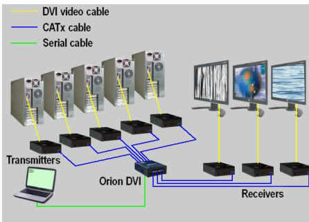
Figure 9. Cross Point Switch - 5 x 3
