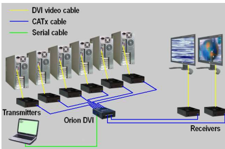
Figure 10. Cross Point Switch - 6 x 2
