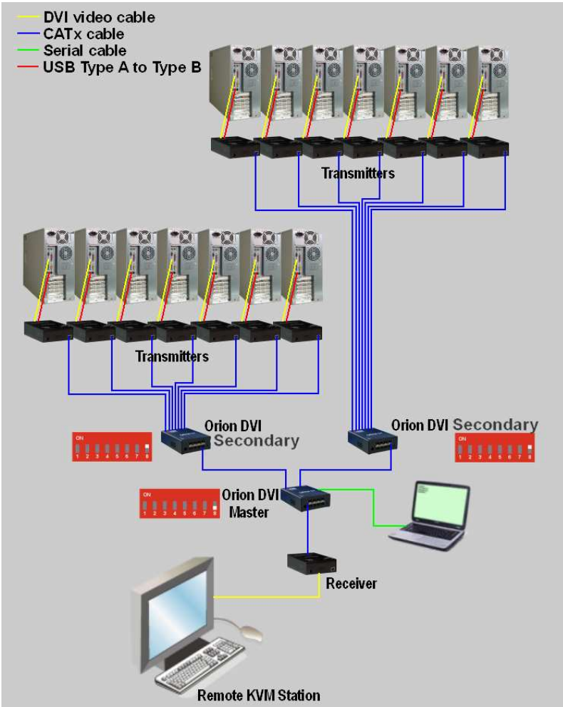
Figure 15. Single Head KVM Switch (Cascaded)
