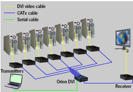
Figure 11. Cross Point Switch - 7 x 1
