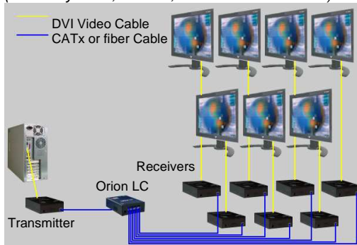
Figure 1. 1x7 Multiplex Receiver
