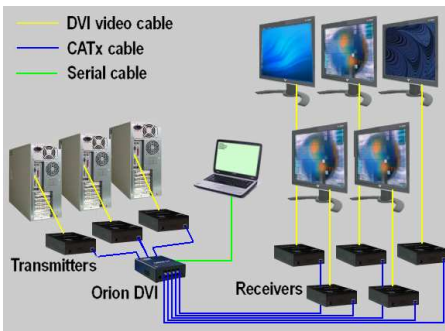
Figure 7. Cross Point Switch - 3 x 5
