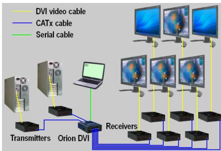
Figure 6. Cross Point Switch - 2 x 6
