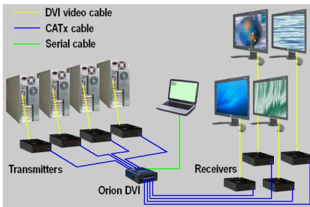
Figure 8. Cross Point Switch - 4 x 4
