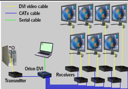
Figure 5. Crosspoint-Switch 1 x 7
