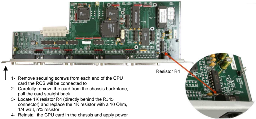
Figure 1. Replacing Resistor R4
